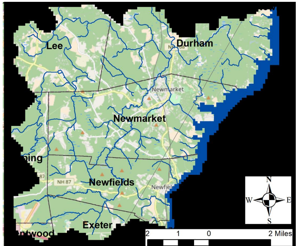
Figure 2. Study area showing streams, constant head (blue) and no flow (black) boundaries [OpenStreetMap contributors, 2016]
