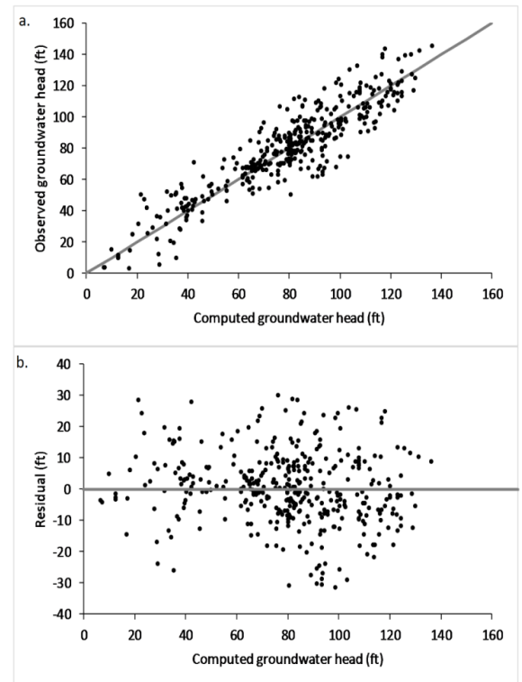
Figure 5. (a) Groundwater heads in observation wells from all 22 layers in the study area versus computed groundwater heads, and (b) groundwater-head residuals (simulated minus observed heads) versus computed groundwater heads.
